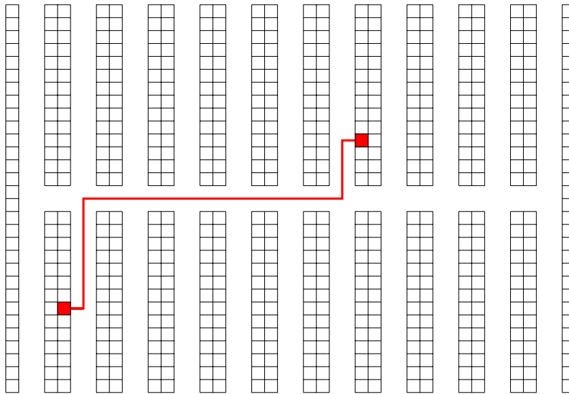
Figure 6.11: A cross-aisle allows more direct and therefore shorter travel between storage locations.
