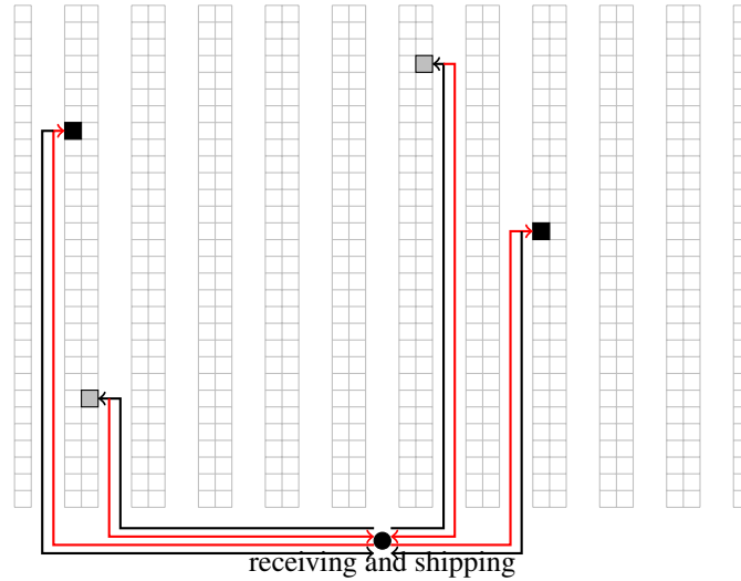
Figure 6.5: Under single-cycle protocol, half of all forklift travel is unproductive (red lines). In this example, both receiving and shipping are at the bottom (black disk). Trips to stow a pallet in an available location (gray squares) require that the forklift return with empty forks. Similarly, any trip to retrieve a pallet from a location (black squares) requires that the journey begin with empty forks.
