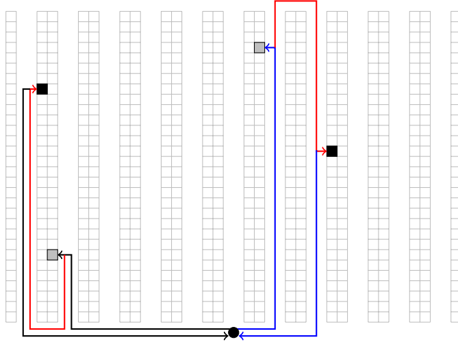
Figure 6.6: Dual-cycles can reduce dead-heading by enabling travel directly from a stow to a retrieval. In this example, each of two stows (gray locations) have been paired with a retrieval (black locations). Dead-heading is shown in red.
