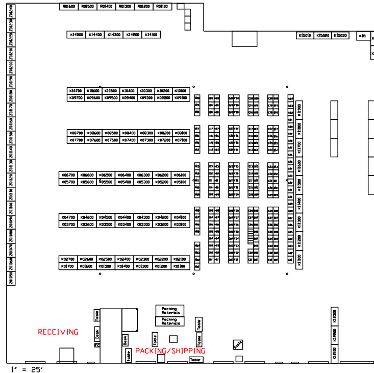
Figure 6.15: Question 6.8: Critique this layout of a service parts distribution center.
